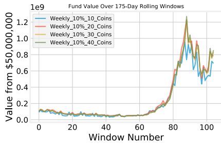
Fig. 5. Portfolio Performance for Different Number of Coins
